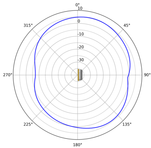
2 GHz Azimuth
