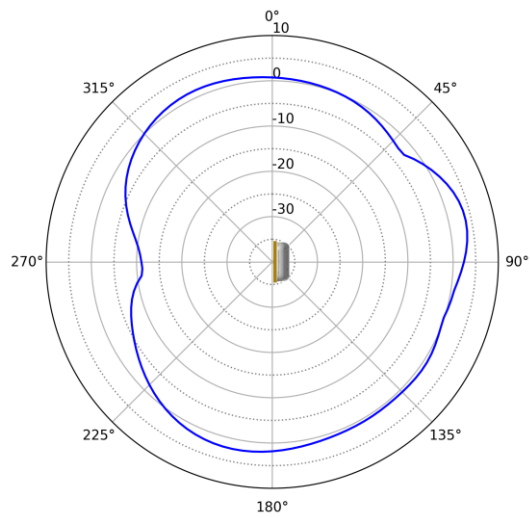
6 GHz Azimuth
