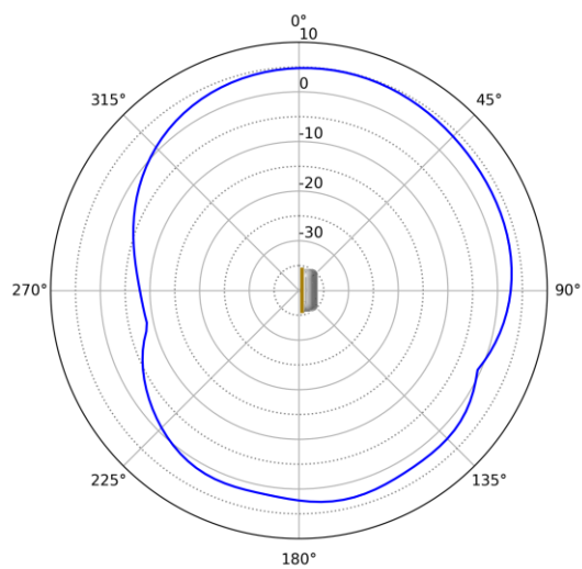
5 GHz Azimuth
