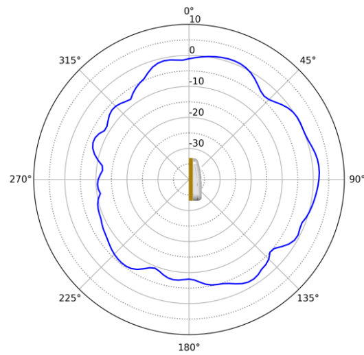
6 GHz Elevation
