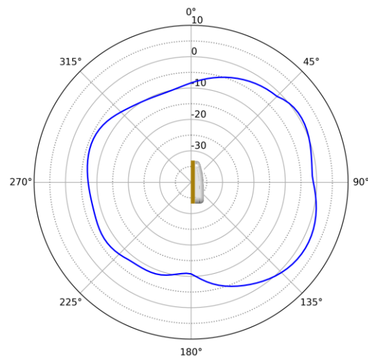
2 GHz Elevation
