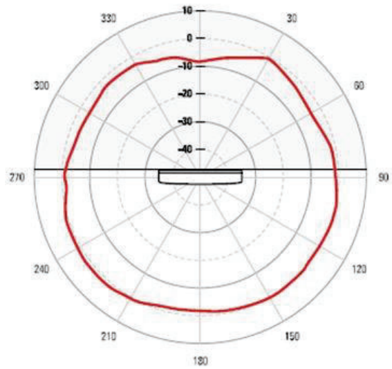
Elevation - 5 GHz
