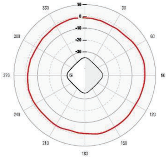
Azimuth - 5 GHz
