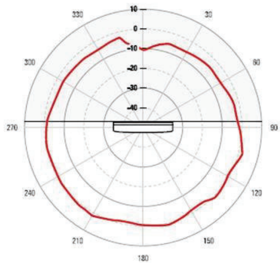
Elevation - 5 GHz
