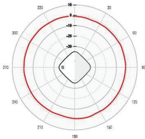
Azimuth - 5 GHz
